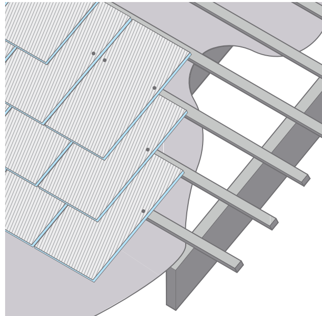
Open Rafter Construction
