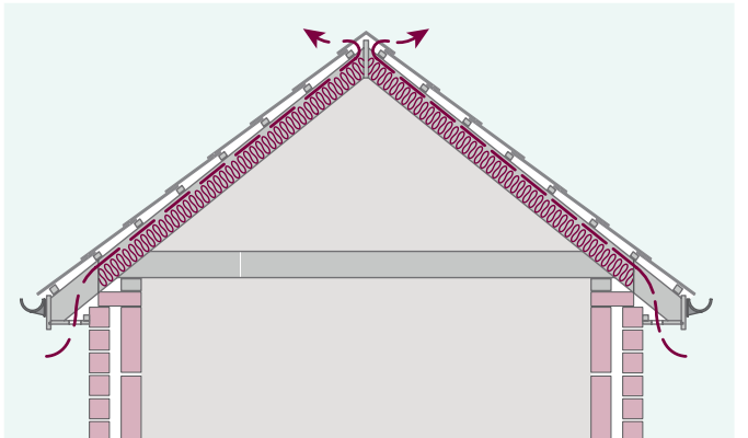
Warm roof insulation at rafter level
