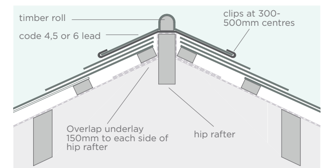
Fixing with ridge lead rop hip
